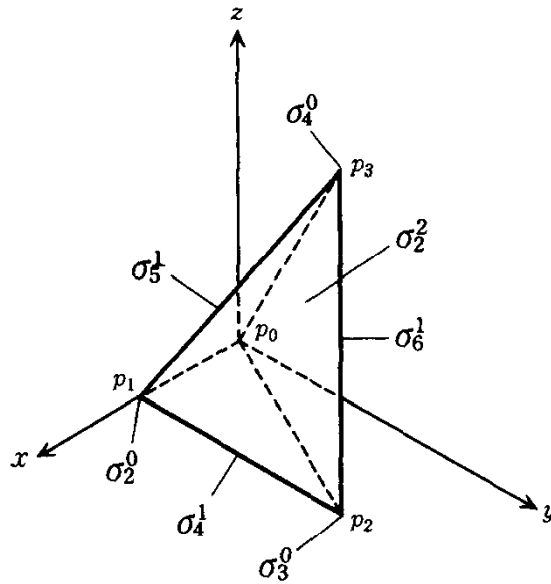
FIGURE 5.1. Simplicial complex
