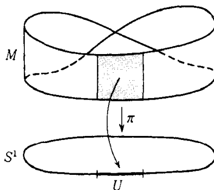
FIGURE 8.2. The Möbius strip
