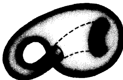
FIGURE 8.3. The Klein bottle
