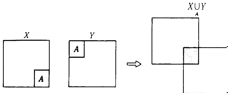
FIGURE 2.2. Topological sum
