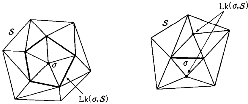
FIGURE 1. Link complex
