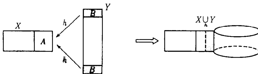
FIGURE 2.3. Attaching space
