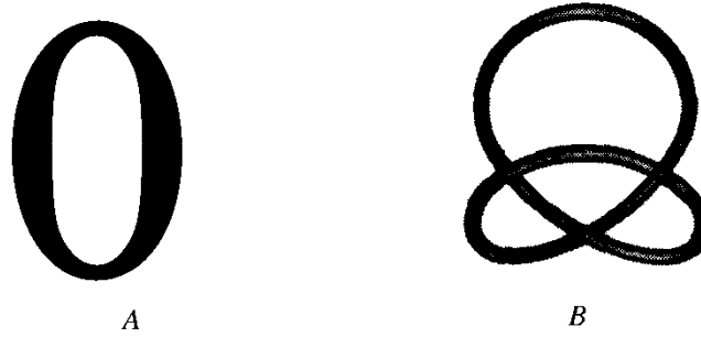
FIGURE 1.2. Knots
