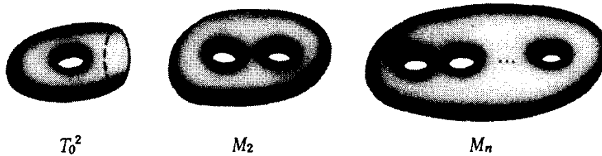
FIGURE 2.4. Closed surfaces
