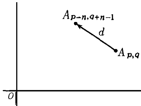
FIGURE 9.1. Differential
